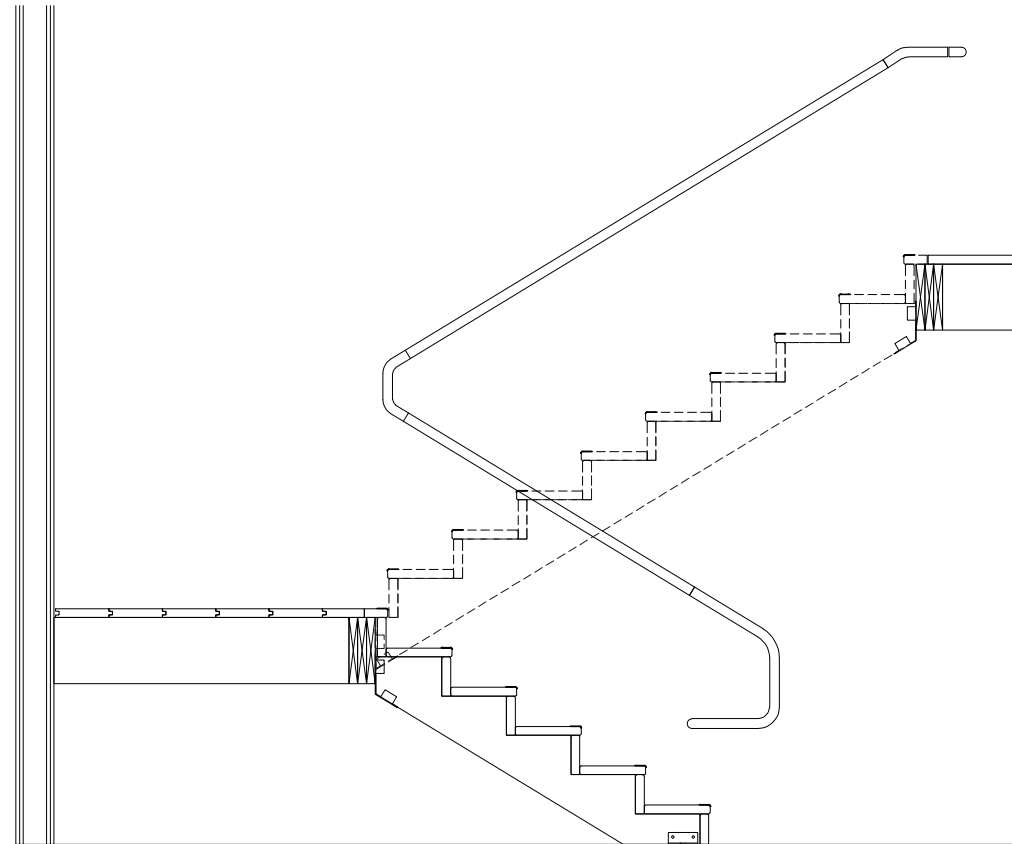
A-1 ELEVATION VIEW
