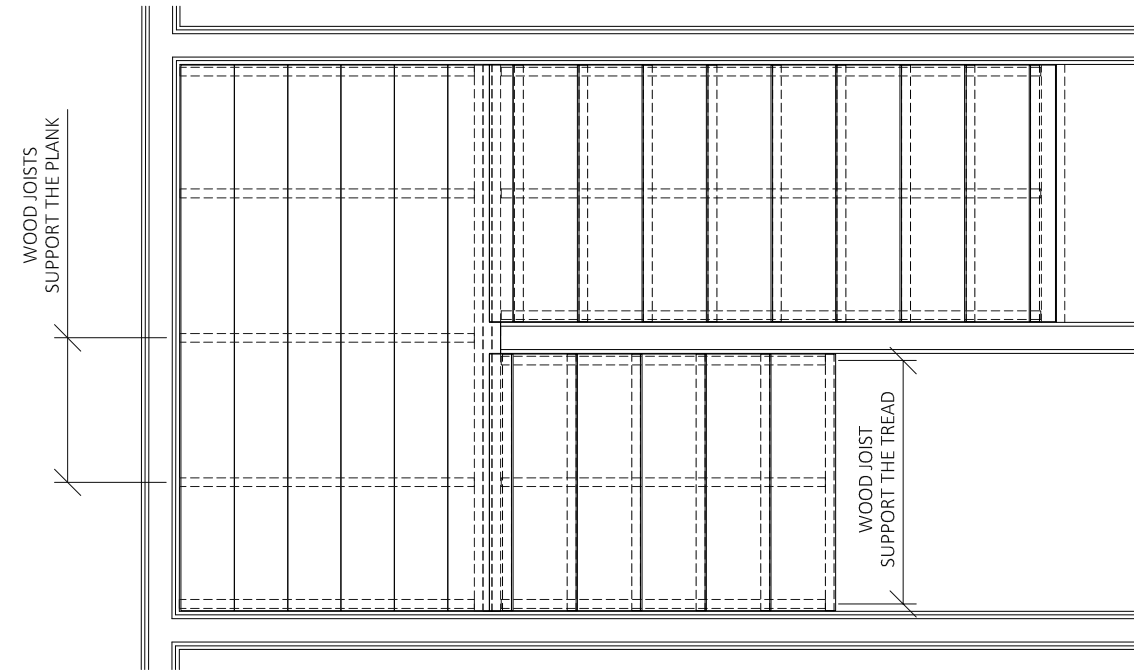
A-2 TOP VIEW
