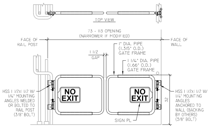
DOUBLE SWING GATE ADJUSTABLE WIDTH - SELF CLOSING - SELF STOPS AT ZERO - HARDWARE INCLUDED INCLUDES PHOTOLUMINESCENT "NO EXIT" SIGN
