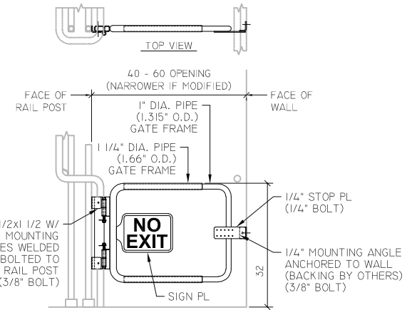
POST MOUNT SWING GATE ADJUSTABLE WIDTH - SELF CLOSING - SELF STOPS AT ZERO - HARDWARE INCLUDED INCLUDES PHOTOLUMINESCENT "NO EXIT" SIGN
