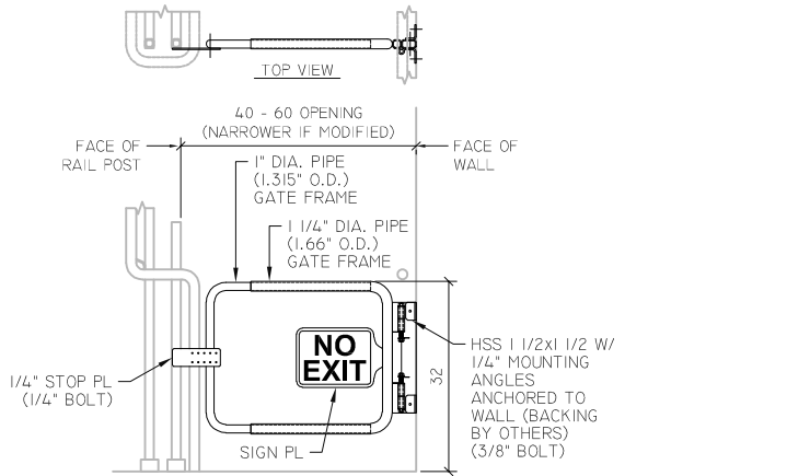
WALL MOUNT SWING GATE ADJUSTABLE WIDTH - SELF CLOSING - SELF STOPS AT ZERO - HARDWARE INCLUDED INCLUDES PHOTOLUMINESCENT "NO EXIT" SIGN
