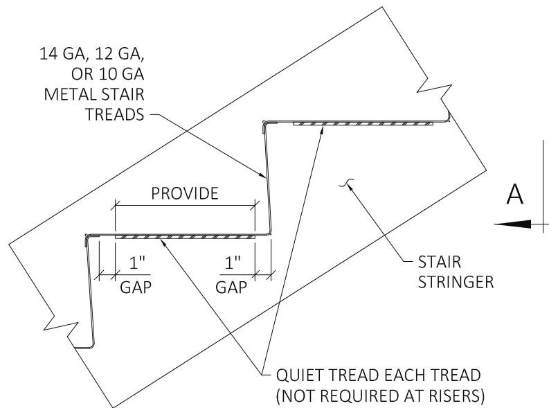
STAIR TREAD/RISER PROFILE VIEW
